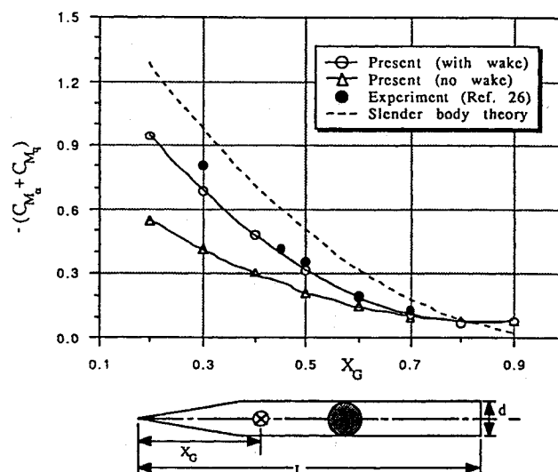
Fig. 4 Effect of the pitching axis location on damping-in-pitch moment for a cone-cylinder body ( L/d = 7.5 ) at M = 0.3 .
