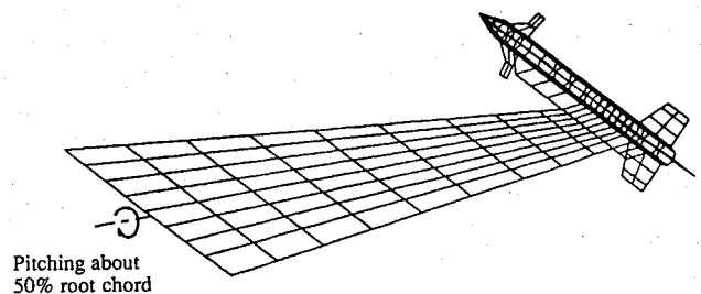
Fig. 16 Northrop F-5 wing with tip missile configuration showing paneling scheme.
