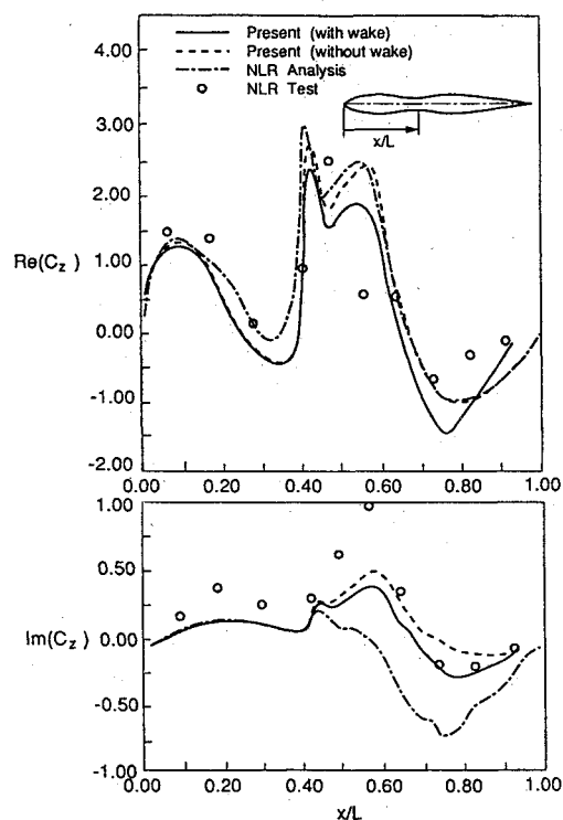
Fig. 10 Unsteady normal load distribution along the tip-tank of NLR wing-tip-tank configuration; M = 0.45 , \alpha = 0 deg, k = 0.305 , and \bar{x}_0 = 0.15c_R .
