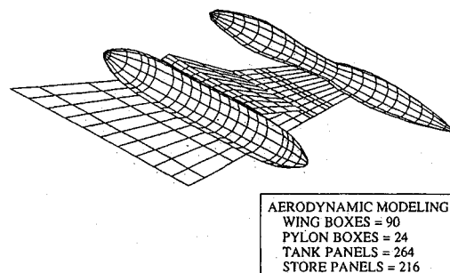
Fig. 11 NLR wing-tip-tank-pylon-store configuration showing paneling scheme.
